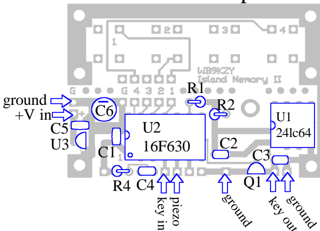
Circuit Board Top View
