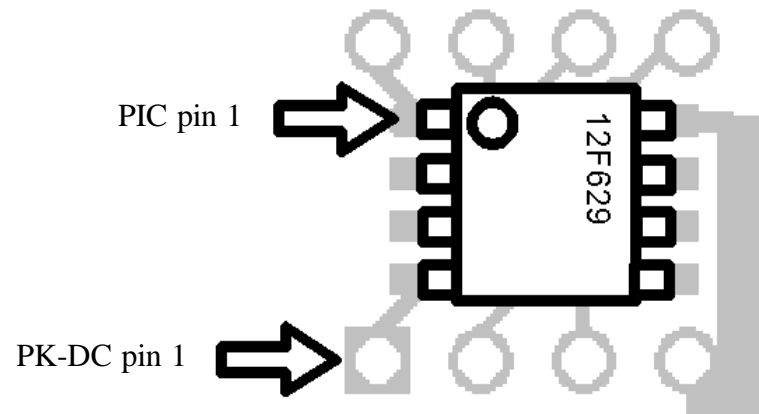
Top View of Circuit Board
